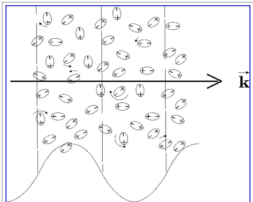
Figure 4. Sketch of the effect of a plane EMR wave propagating in a bulk fluid of polar elements, with a net result of increasing the temperature. The E -vector magnitude and polarity (+ up) is shown on an arbitrary vertical scale drawn through nodes of the wave; the horizontal scale is for illustration only. The EMR torque on a few of the polar elements is shown as a vector in the \pm \vec{H} direction.
